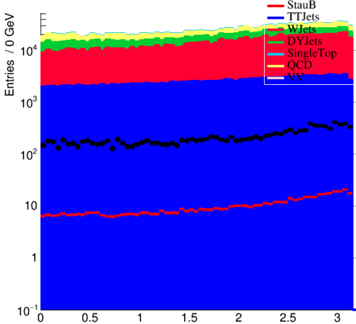
dPhiJMET Trigger
