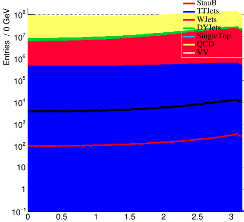
dPhiJMET $tau_h$
