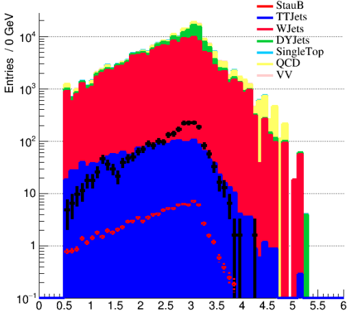
dR_mutau ZMass cut
