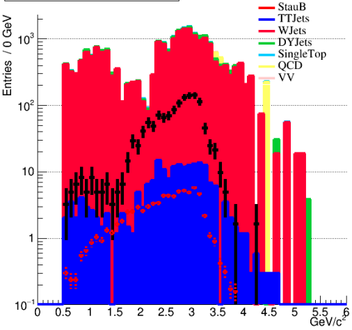
dR_mutau dPhi > 1
