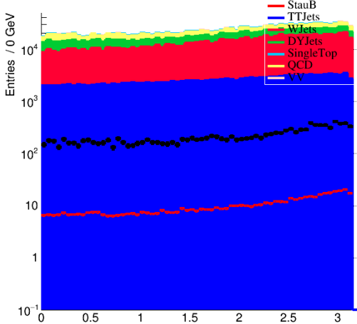
dPhiJMET 2nd lept-Veto
