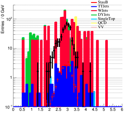
dR_mutau dPhi > 1
