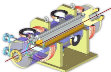
mirror chamber
