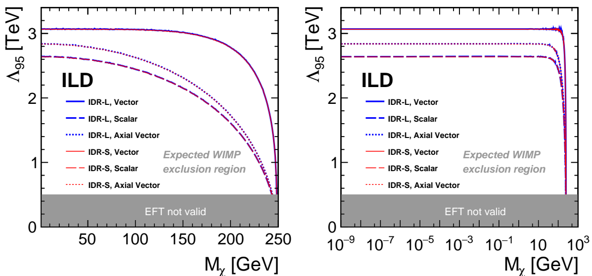
Figure 20: 95% confidence level exclusion limits for different effective operators with the luminosity sharing described in Tab. 4.
