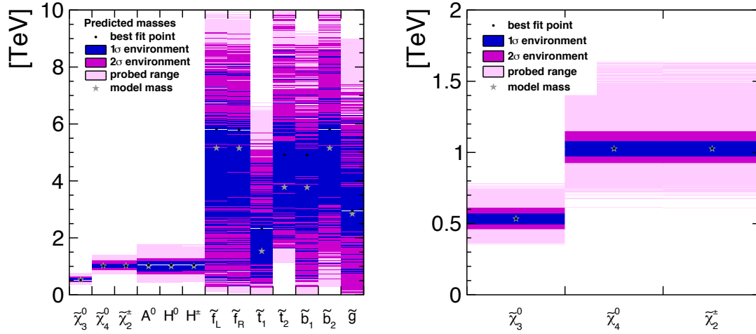
Figure 3: Predicted mass ranges from the fit to ILC2. Left: pMSSM-10 fit, Right: pMSSM-4 fit.
