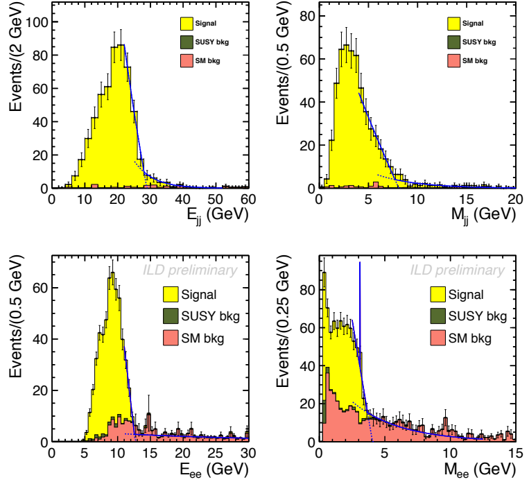
Figure 2: Energy and mass distributions for jet-jet in ILC2 ( top, left and right); and for e\text{-}e in nGMM1. (bottom, left and right)
