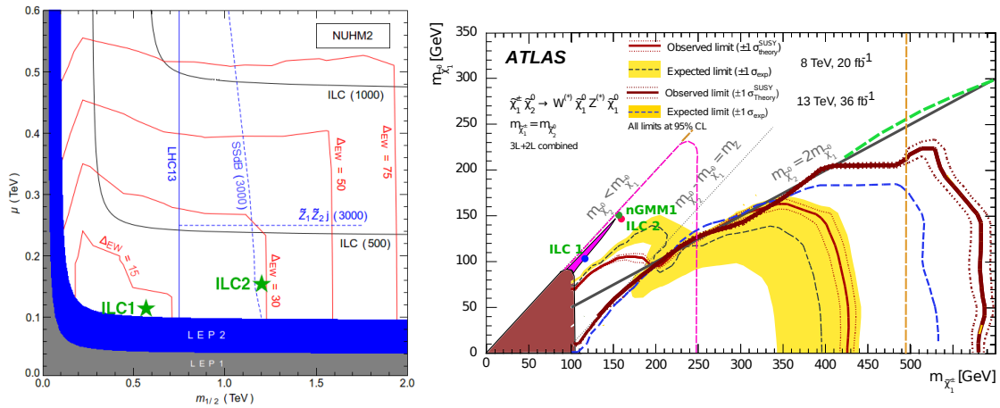
Figure 1: Model-parameter space, with our benchmarks indicated. Left: The m_{1/2} vs. \mu plane in the NUHM2 model, with projected LHC and ILC reaches. Right: Discovery or exclusion regions in the M_{NLSP} - M_{LSP} plane for a \tilde{\chi}_1^\pm . The brown area and the magenta and orange lines show the reaches for e^+e^- colliders (LEP-II, ILC@500, ILC@1000) together with current-LHC limits, and HL-LHC projections (green dashed). The magenta area is the ATLAS low \Delta_m exclusion, which however is in a different model.
