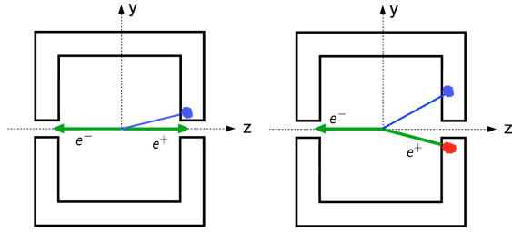
Figure 2 – Sketch of Bhabha scattering events in the detector. With a low p_T photon the leptons tend to go down the beam pipe (left) and the event is indistinguishable from a mono-photon WIMP signal. With the signal requirement of a minimum p_T one of the leptons can be reconstructed in the detector (right).
