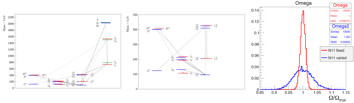
Figure 9 – Left: Spectrum of supersymmetric particles in STC8. Right: The fitted dark matter relic density \Omega reproduces the model value \Omega_{true} . The better the knowledge of the neutralino mixing the smaller the uncertainty.
