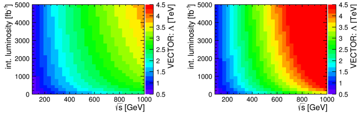
Figure 5 – Testable energy scale \Lambda as a function of the centre-of-mass energy and the integrated luminosity, left (right) without (with) beam polarisation.
