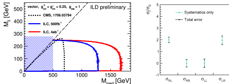
Figure 6 – Left: Comparison of CMS and ILC exclusion limits for a vector operator. Right: Determination of the fully polarised cross-sections for 500 \text{ fb}^{-1} . The chirality of the vector-like operator can be tested.
