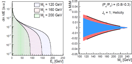
Figure 7 – Left: Photon energy spectrum for different WIMP masses. Right: Uncertainty of the fitted WIMP mass as a function of WIMP mass in the framework of a vector effective operator. The systematic uncertainties (blue) dominate in this conservative approach where it is assumed that no information on the beam spectrum is available.
