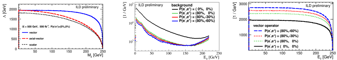
Figure 4 – Exclusion limit on the energy scale \Lambda as a function of the WIMP mass for different effective operators (left). Number of background events for 500\text{ fb}^{-1} (centre) and sensitivity (right) for different beam polarisations.
