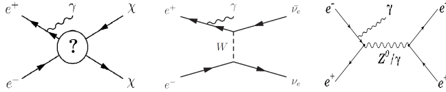
Figure 1 – Visualisation of the signal process and example Feynman diagrams for the two main background processes: radiative neutrino pair production and Bhabha scattering.
