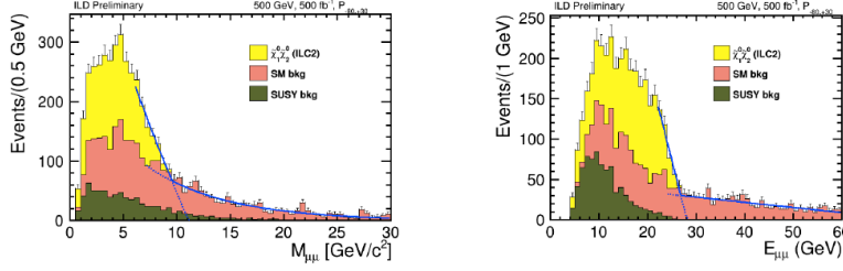
Figure 8 – The di-muon invariant mass (left) and di-muon energy (right) distributions for ILC2 and 500 \text{ fb}^{-1} .
