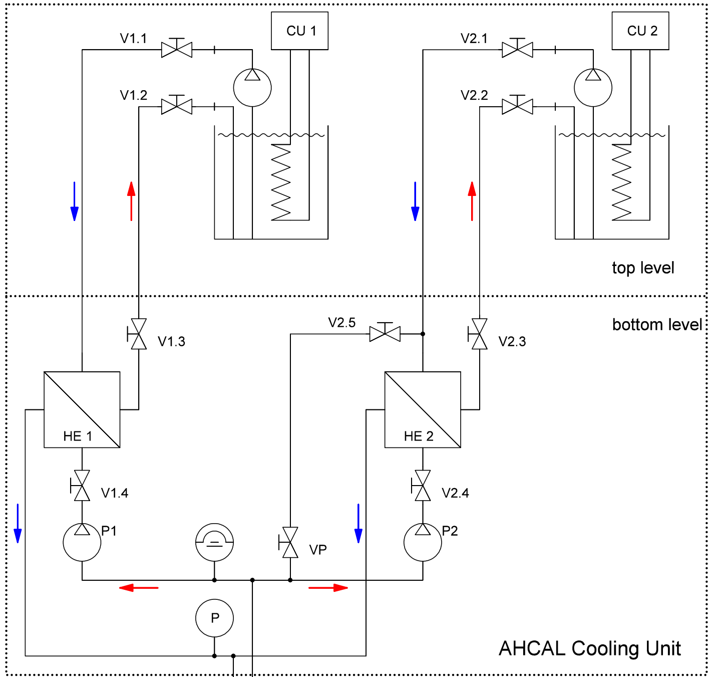
AHCAL Cooling System - Flow Diagram (overpressure)
